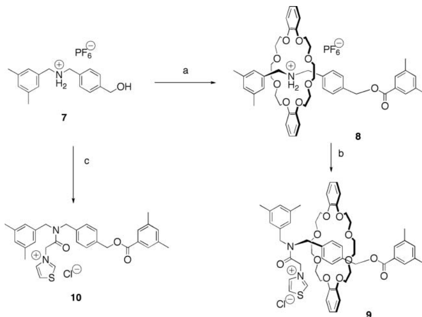
Scheme 2 Preparation of rotaxane 9 and non-rotaxane 10 catalysts. (a) DB24C8, 3,5-dimethylbenzoic anhydride, Bu 3 P, CH 2 Cl 2 , r.t., 81%; (b) 1. Chloroacetic anhydride, Et 3 N, DMF, 40°C, 48 h, 76%; 2. thiazole, NaI, r.t., 3 d; 3. Amberlite IRA-400 (Cl-type), 92% (2steps); (c) 1. Chloroacetic anhydride, THF, -40°C, 16 h, 74%; 2. 3,5-dimethylbenzoic anhydride, Bu 3 P, CH 2 Cl 2 , r.t., 8 h, 84%; 3. thiazole, NaI, r.t., 3 d; 4) Amberlite IRA-400 (Cl-type), 99% (2 steps).
